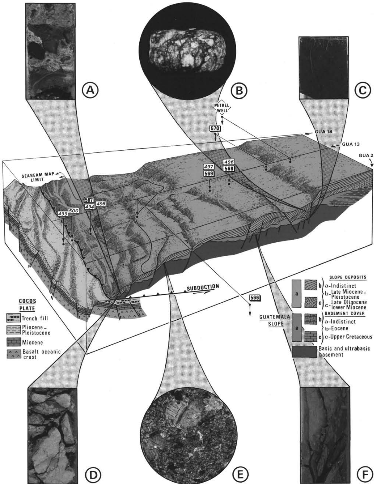
A. Sample 567-18, CC: piece of Miocene sediment below serpentinite blocks. B. Core 570-27: solid Miocene gas hydrate. C. Section 570-41-3: serpentinitized peridotite from the upslope basement. D. Section 567-19-1: Upper Cretaceous limestones above an ophiolitic complex comprising slope basement. E. Sample 566-6-1, 31-33 cm: serpentinitized peridotite in the basement (petrographic section). F. Section 569-9-1: late Eocene mudstone.
