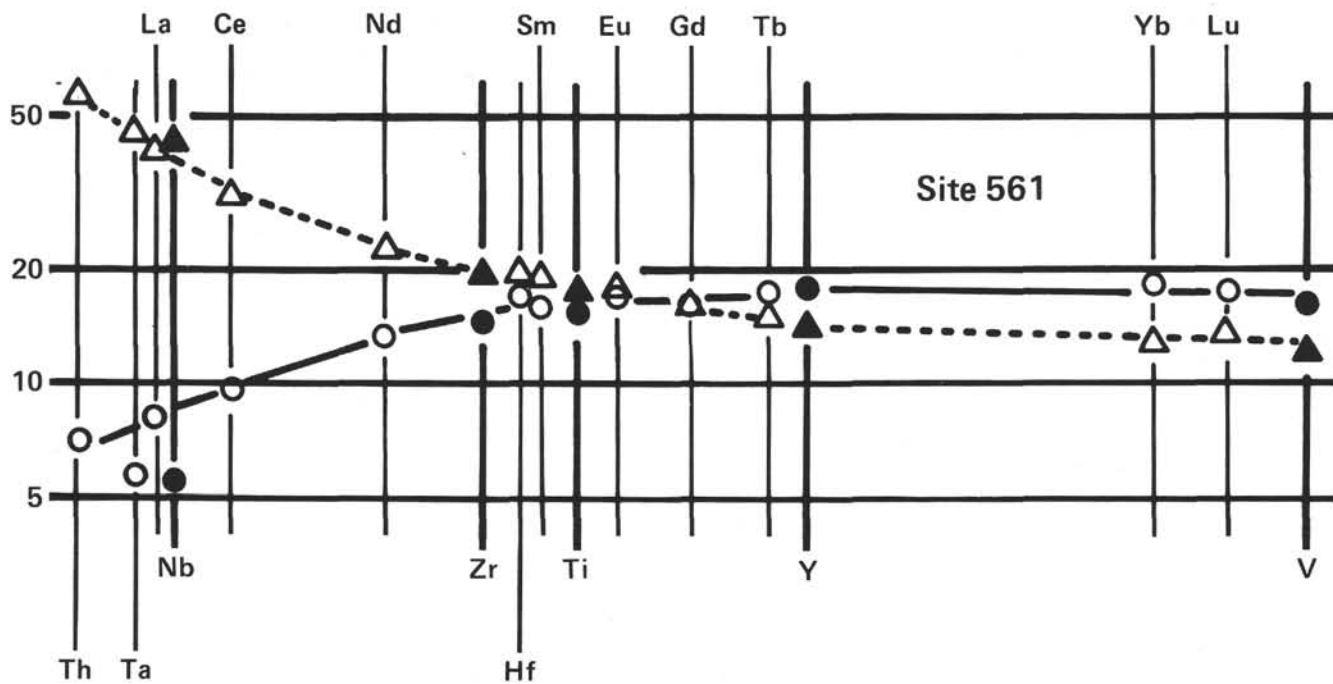
Crossing patterns of hygromagmaphile elements in basalts from Site 561. Such crossing patterns, also found at Site 558, reflect mantle heterogeneity and/or different extents of partial melting of mantle material. The ordinate corresponds to the concentrations of the elements in basalts normalized to their concentrations in chondrites. The rare earth elements are plotted versus their atomic numbers (upper part of the figure); the non-rare earth elements are plotted according to their similarity to rare earth elements with respect to magmatic processes (lower part of the figure). Nb, Zr, Ti, Y, and V (filled symbols) correspond to ship-board data (see Etoubleau et al., this volume, for analytical chemistry on board) that were used for conducting the cruise. The other elements (open symbols) correspond to onshore data from several references in this volume (Bougault et al., Rideout and Schilling, Weaver et al., Drake et al., Hertogen et al.).
