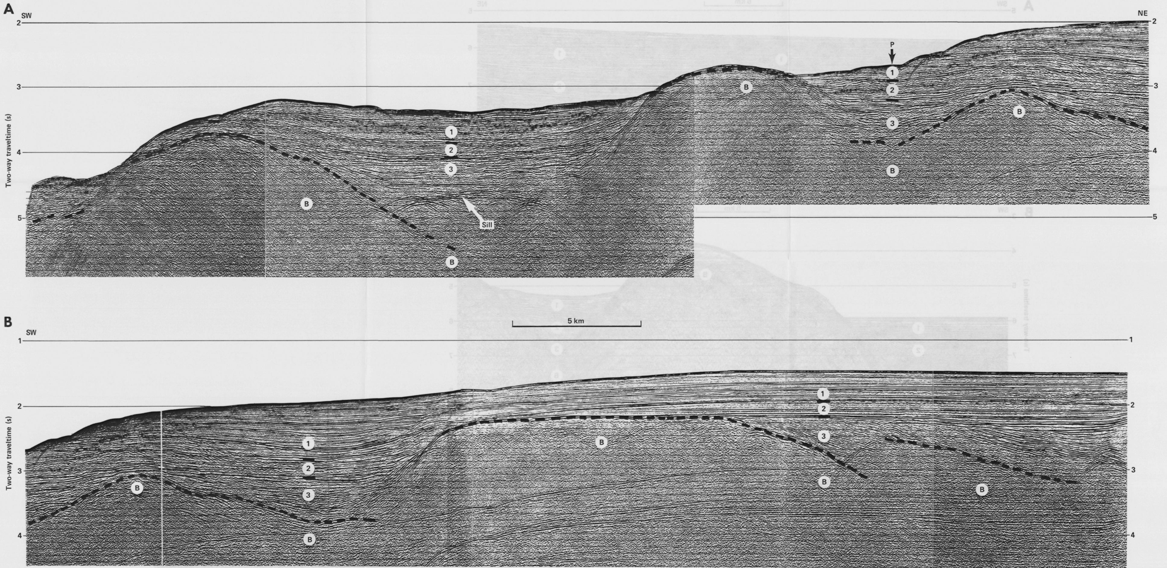
Volume 80: Chapter 54: Figure 10. Unmigrated seismic profile across a series of tilted blocks on the southern flank of Goban Spur. Section A is southwest part of profile, Section B the northeast part (seis-stratigraphic sequences as described in text). Note the sill in the deep half-graben toward the southwest end of the profile. Profile located on Figure 2. P = point of overlap of two parts of profile.
