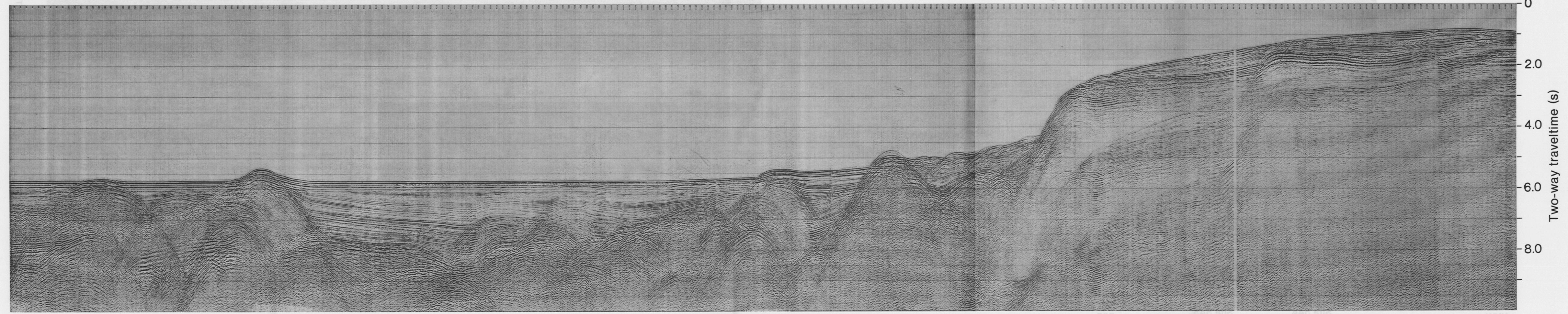
Volume 79: Chapter 38: Figure 8. Multichannel seismic line 1/4 79-02.
