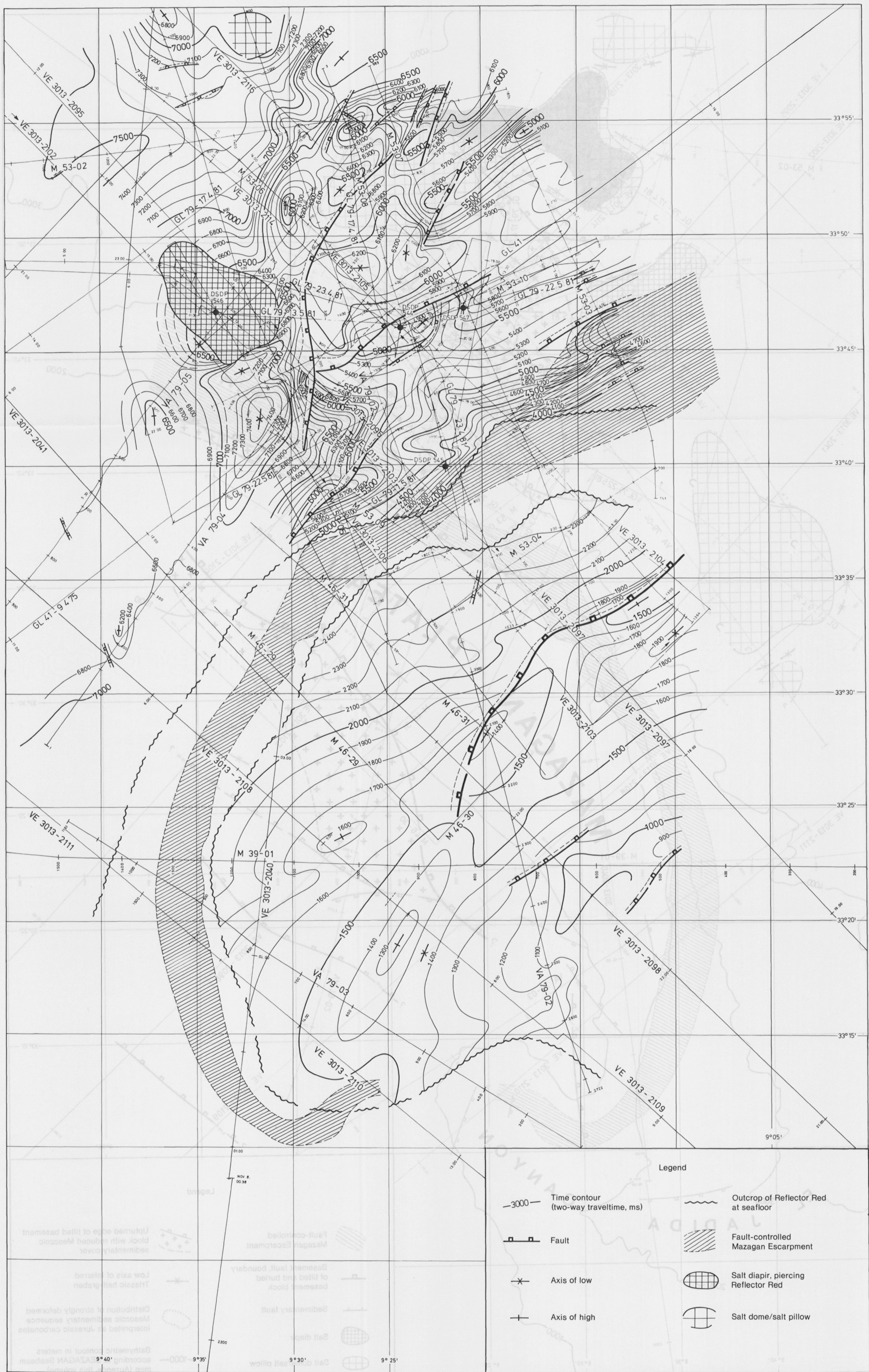
Volume 79: Chapter 38: Figure 11. Time contour map of Reflector R (Tertiary/Cretaceous [Cenomanian] boundary) in the area of DSDP Leg 79, including the Mazagan Plateau.
