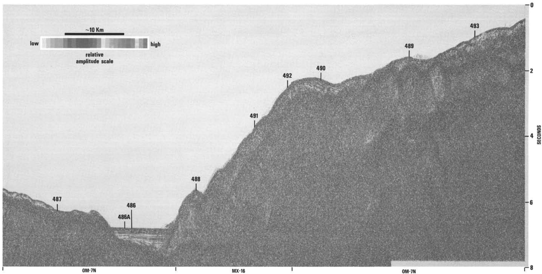
Composite cross section through Leg 66 drill sites combining parts of Seismic Lines OM-7N and MX-16. Displays by Gulf Science and Technology Company.
