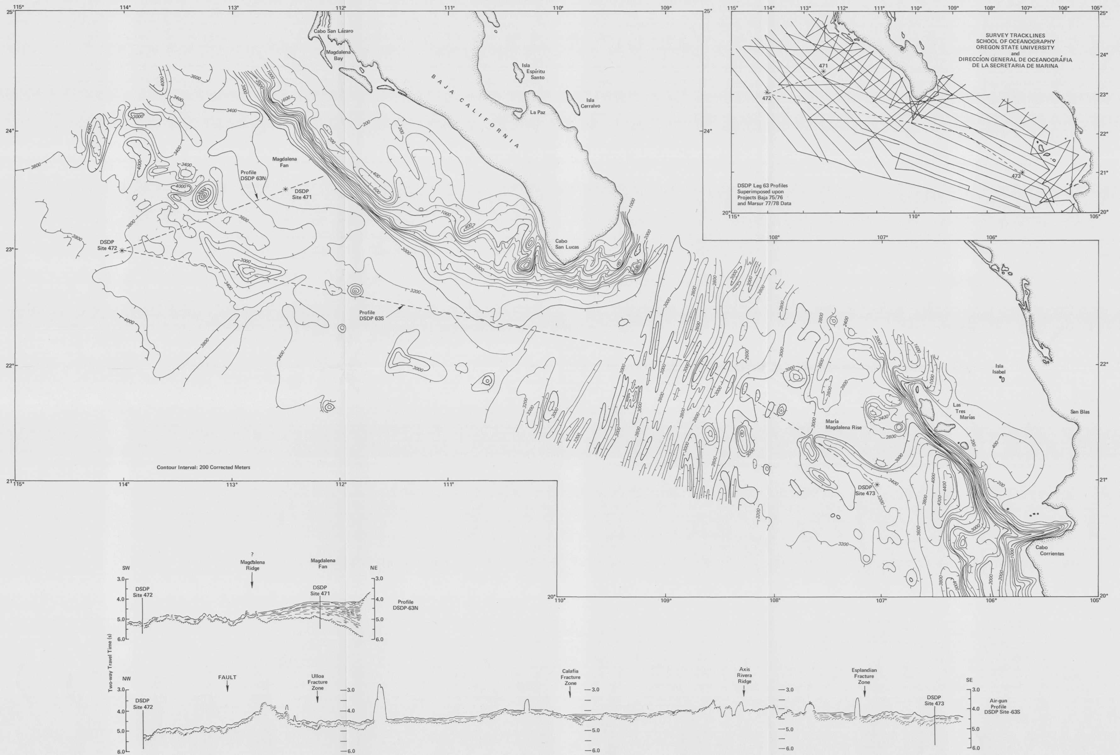
Volume 63: Chapter 38: Figure 1. Bathymetry and DSDP Leg 63 seismic reflection profiles at the mouth of the Gulf of California. (Inset shows survey track lines used to prepare the map.)
