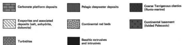
Schematic interpretation of the continental margin off Morocco during the Triassic and Jurassic .
