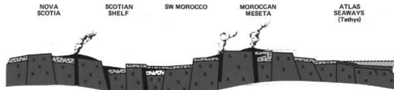
I. LATE TRIASSIC–EARLIEST JURASSIC
