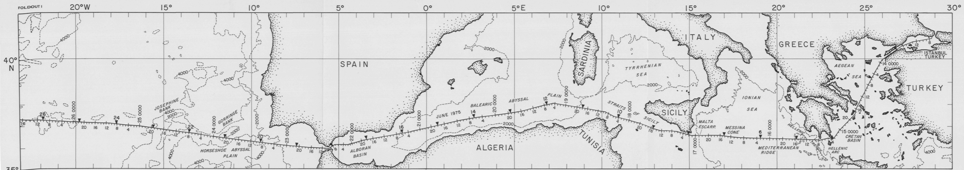
GLOMAR CHALLENGER LEG 43 (13 JUNE - 12 AUGUST, 1975) - CONTOUR INTERVAL 2000 m
