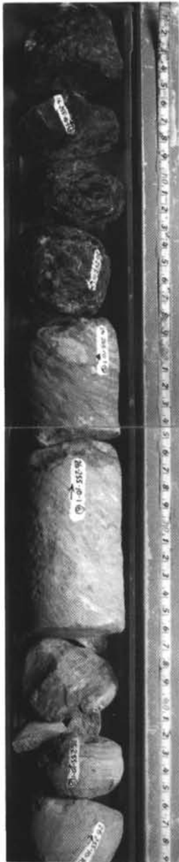
CRETACEOUS CHERT AND LIMESTONE FROM BROKEN RIDGE (SITE 255, CORE 10)
