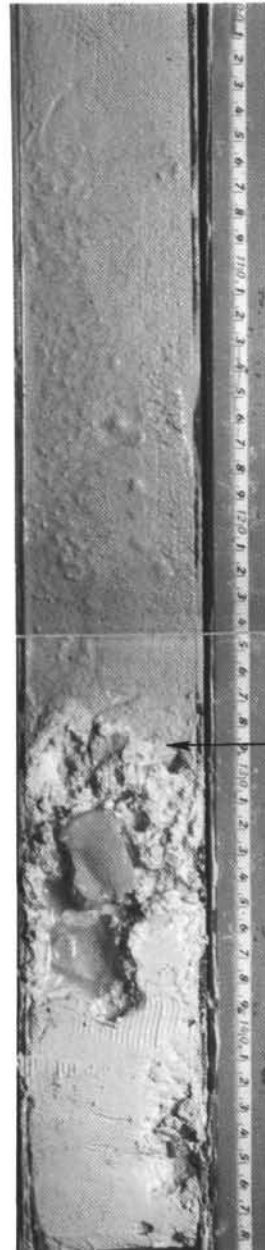
CRETACEOUS – TERTIARY UNCONFORMITY FROM NATURALISTE PLATEAU (HOLE 258A CORE 8)
