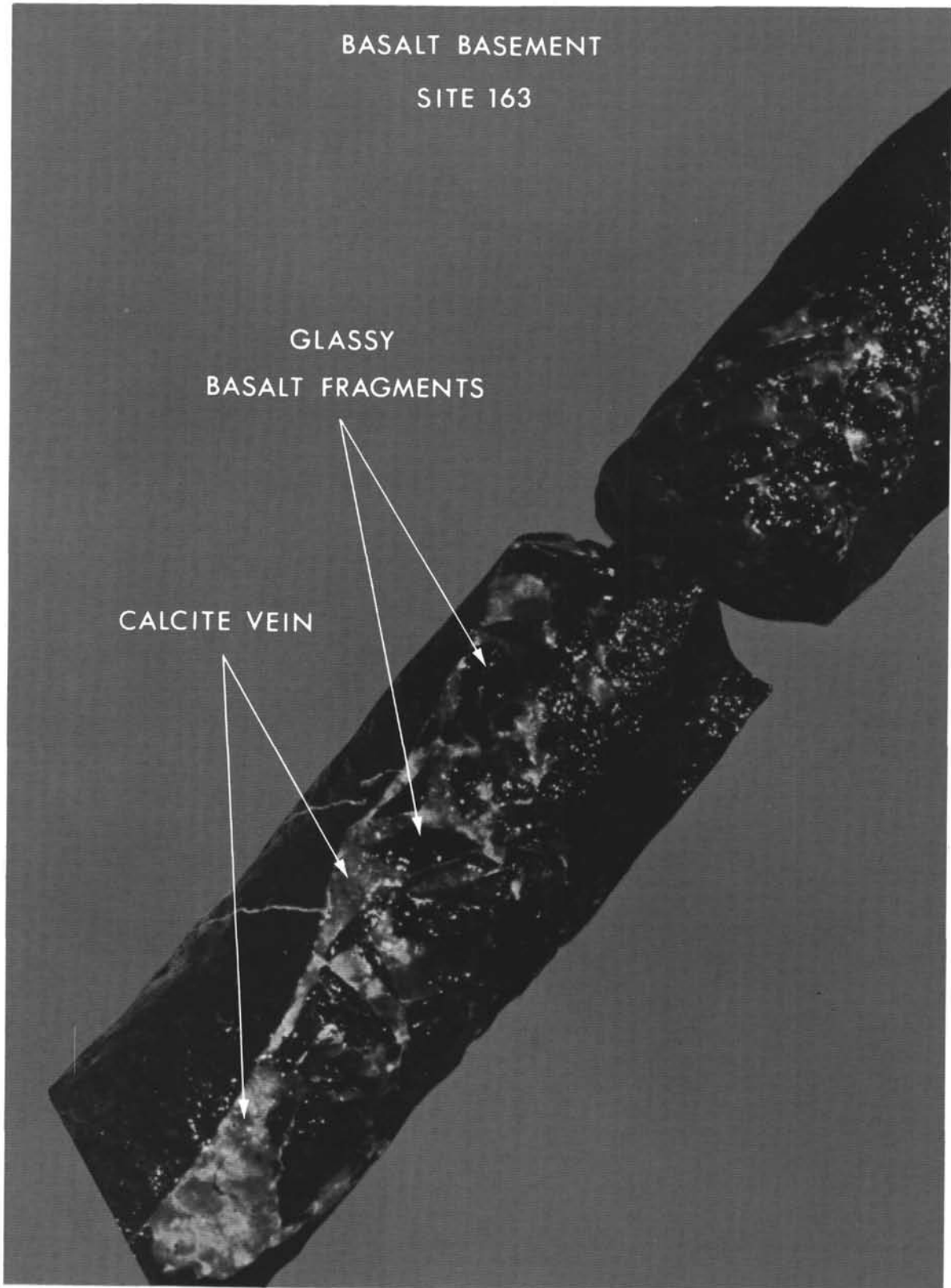
Greenish gray calcite vein containing angular fragments of glassy basalt. Most of the fragments are quite fresh. This vein is about 10 meters below the sediment-basalt contact and lies between the 5th and 6th of seven cooling units cored at Site 163. 163-29-1 (120-143 cm)
